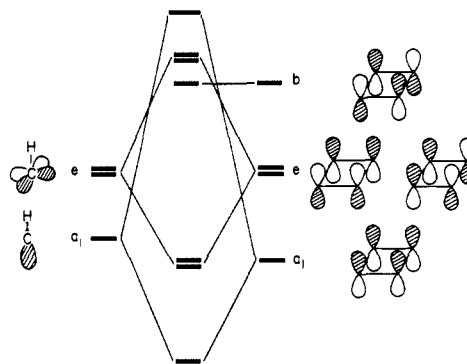
Figure 5. Interaction diagram showing how the orbitals of a C_{4v} (\text{CH})_5 are constructed from a CH and a cyclobutadiene. Note that this is not a correlation diagram for the approach of \text{CH}^+ to (\text{CH})_4 .
